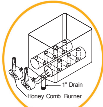
Tube-Fire Heating System for FSGDF 12 & FSGDF 11D
